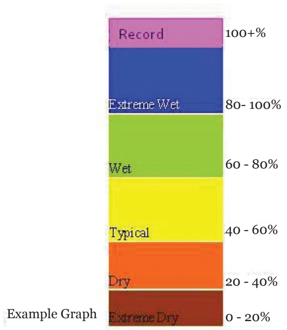
Fig. 3. A proposed sample template for a new precipitation amount graphic.
