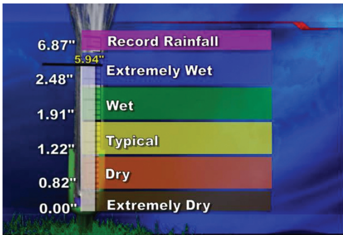
Fig. 4. A second proposed sample template for a new precipitation amount graphic with data from January 2005.
