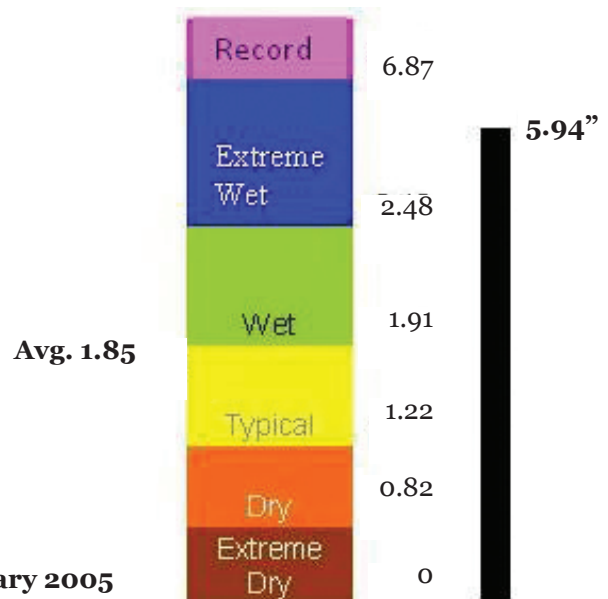
Fig. 5. The generic template from Fig. 3 with data from January 2005. All precipitation amounts are shown in inches.
