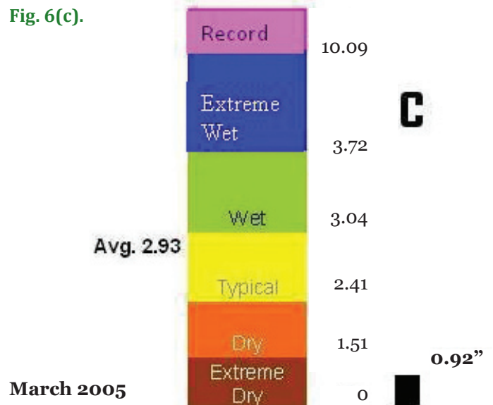
Fig. 6. As in Fig. 5, except for March 2005. This figure shows a monthly progression for a) March 10, b) March 20, and c) the end of the month.
