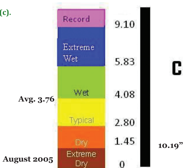
Fig. 7. As in Fig. 5, except for August 2005.
