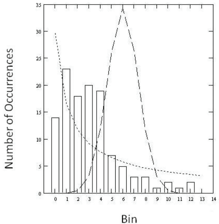
Fig. 1. Binned monthly precipitation amounts (bars) for each January from 1890 – 2007. The first bin on the left is monthly precipitation amounts from 0 – 0.50 inches, and each bin is successively 0.50 inches greater. The dotted line represents a fitted gamma distribution, while the long dashed line represents a normal or Gaussian distribution.
