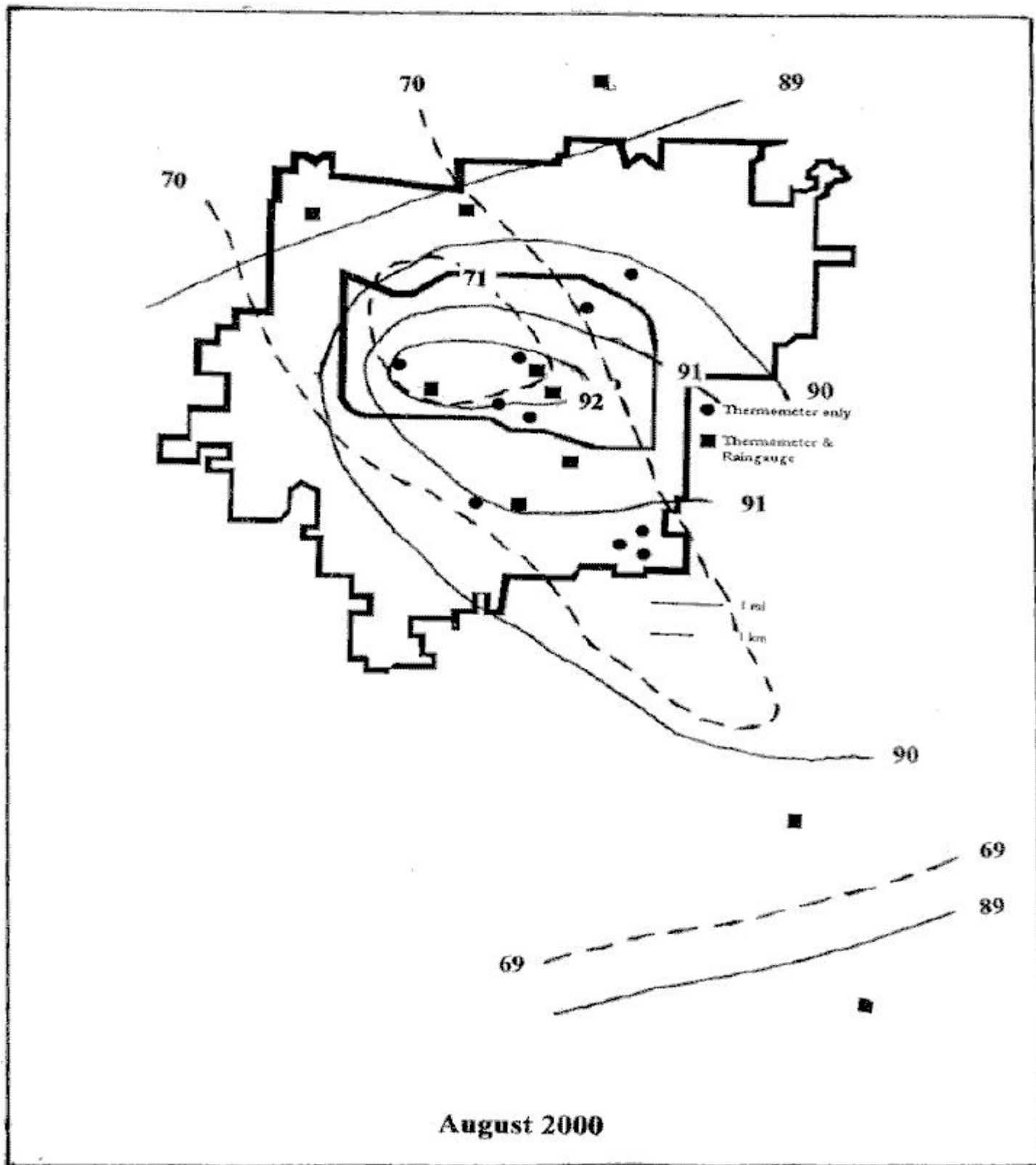
Figure 4. A contour map of monthly mean maximum (solid) and minimum (dashed) temperatures (°F) for August 2000.
